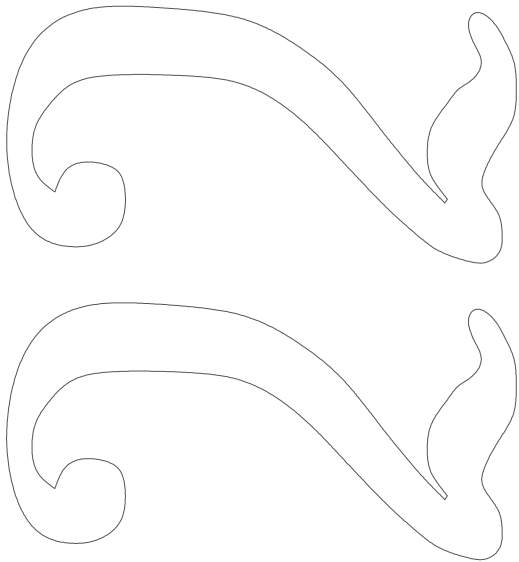
FUSELAGE PORT SIDE
