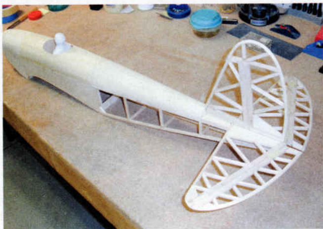
Fuselage and tail surfaces assembled together to check alignment.
