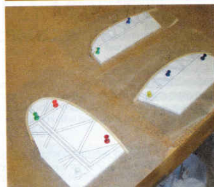
To make the laminations for the tail surfaces, make the forms from foam board. Here the formed parts are shown ready to be removed.
