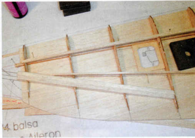
Basic wing assembly is shown here. Notice the aileron servo mount detail.
